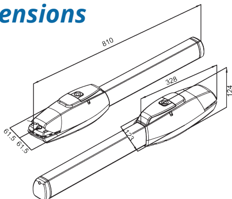
iS300 Dual Swing Motors with Built-in Stopper.
